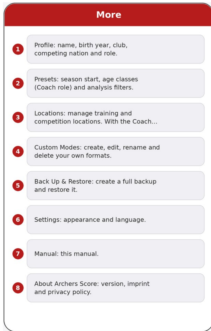
Figure 23: More
