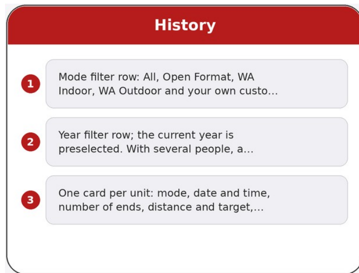
Figure 18: History
