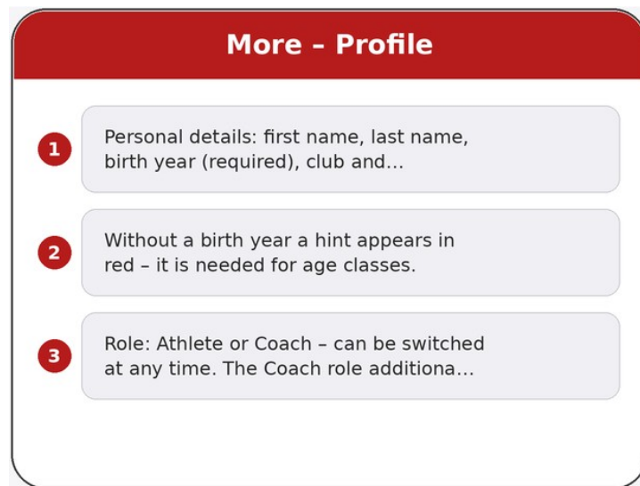
Figure 1: More - Profile
