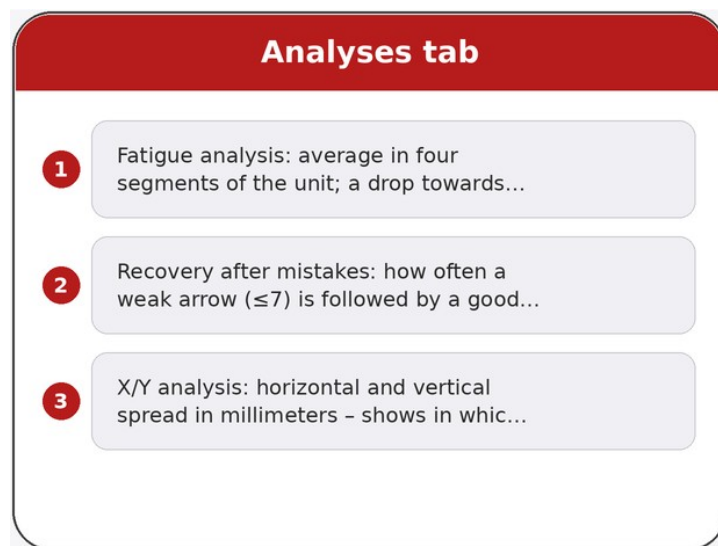
Figure 22: Analyses tab
