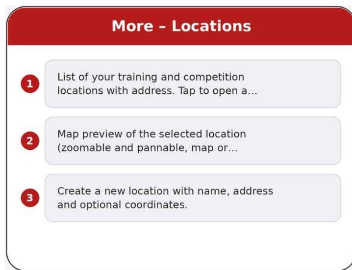
Figure 4: More - Locations
