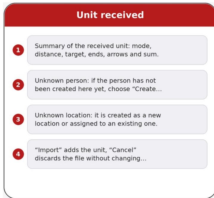
Figure 29: Unit received
