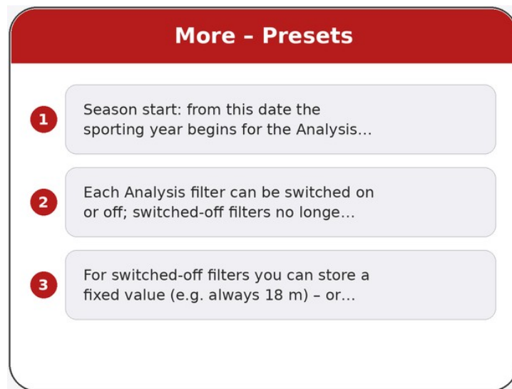
Figure 3: More - Presets
