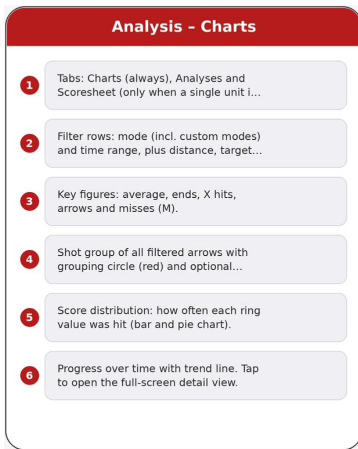
Figure 20: Analysis - Charts
