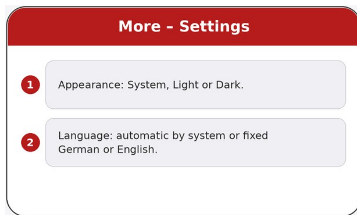
Figure 2: More - Settings
