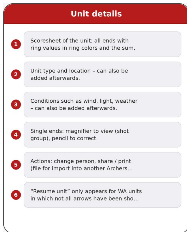
Figure 19: Unit details
